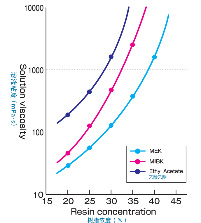
Viscosity of SOLBIN CL solutions in various solvents SOLBIN CL的各种溶剂溶液粘度
