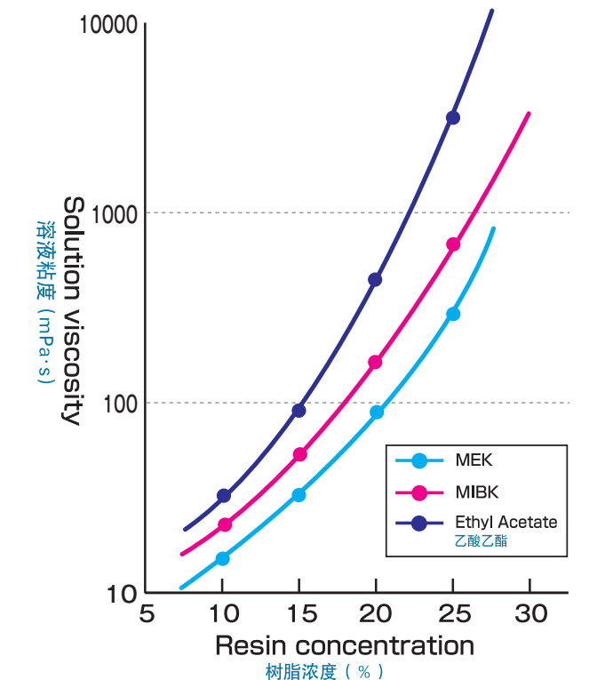
Viscosity of SOLBIN A solutions in various solvents SOLBIN A的各种溶剂溶液粘度
