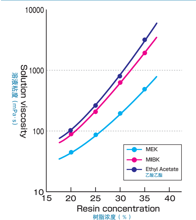
Viscosity of SOLBIN TA5R solutions in various solvents SOLBIN TA5R的各种溶剂溶液粘度
