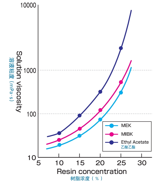
Viscosity of SOLBIN C solutions in various solvents SOLBIN C的各种溶剂溶液粘度
