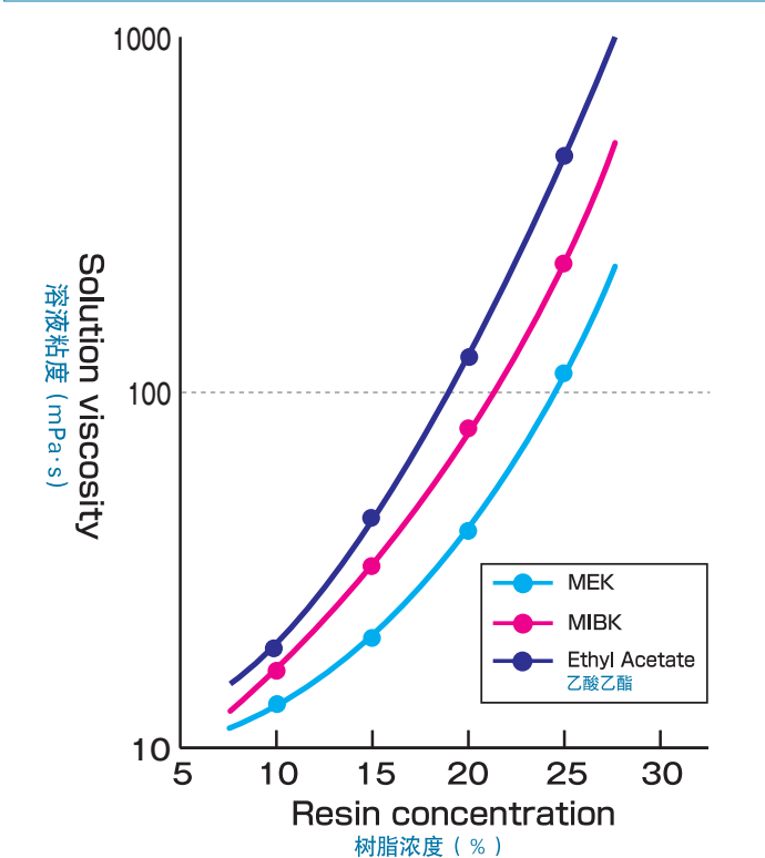
Viscosity of SOLBIN M5 solutions in various solvents SOLBIN M5的各种溶剂溶液粘度
