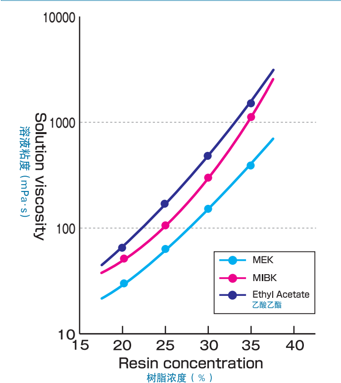
Viscosity of SOLBIN C5R solutions in various solvents SOLBIN C5R的各种溶剂溶液粘度
