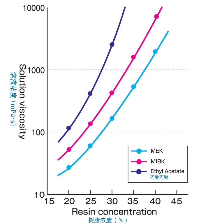
Viscosity of SOLBIN AL solutions in various solvents SOLBIN AL的各种溶剂溶液粘度
