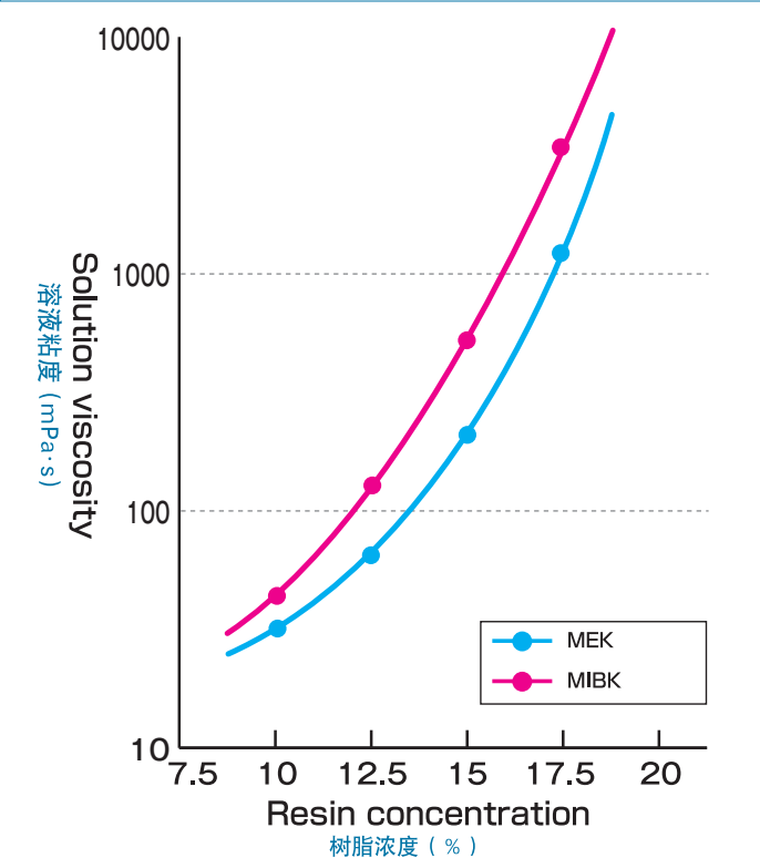
Viscosity of SOLBIN CN solutions in various solvents SOLBIN CN的各种溶剂溶液粘度
